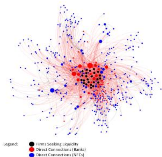
Figure B: 1 st and 2 nd Level Contagion Map
