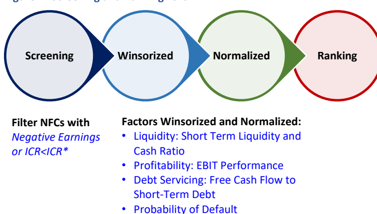
Figure A: Screening and Ranking LSFs
